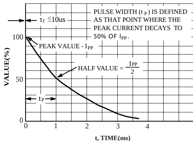
FIG.5 Pulse Waveform
